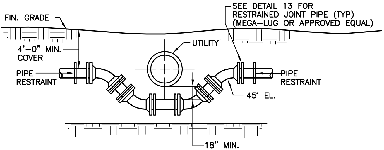
USING ELBOWS
